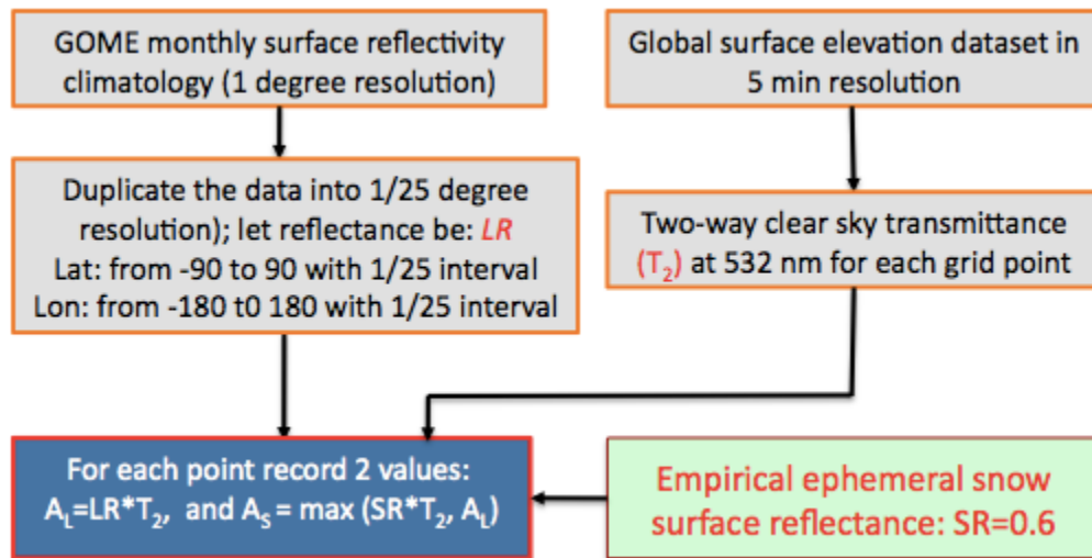
Figure 4.6.6. Flow chart for generating the initial clear sky ASR dataset. There will be one such dataset for each month of the year. Data set does not change from year to year.
