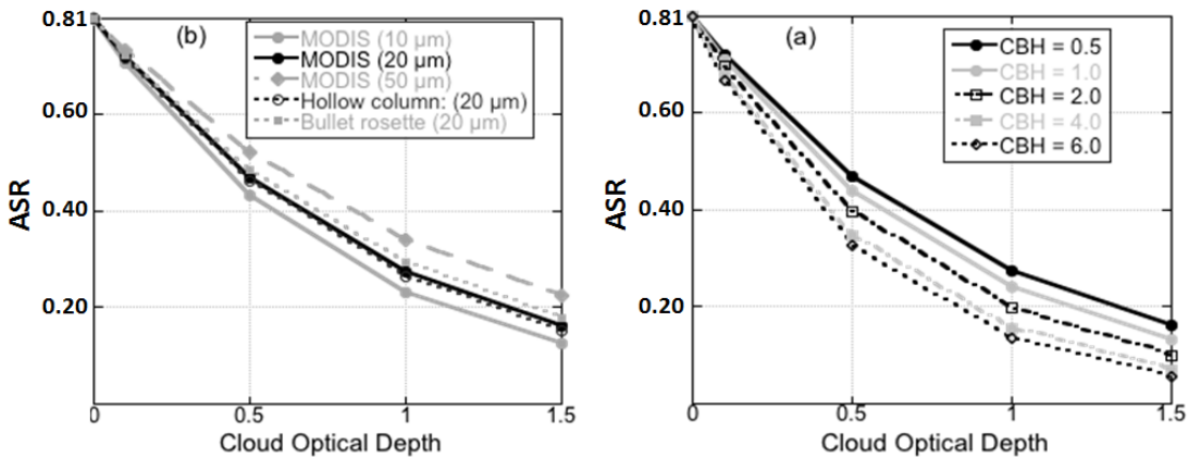
Figure 4.6.2. The effect of cloud properties on ICESat-2 ASR. Results are from Monte Carlo simulations over a surface of reflectivity 1. Telescope of field of view (FOV) is 40 m in diameter. (a) ASR changes as a function of COD for different cloud base heights (CBH) (in km). Cloud thickness is assumed to be 0.5 km; MODIS ice phase function for particle effective radius r_e=20 \mu\text{m} is used. (b) Same as (a) but for different cloud particle sizes and shapes. The numbers in the parentheses in the legend are the effective radii. Clouds are assumed to be located at 0.5 - 1.0 km.
