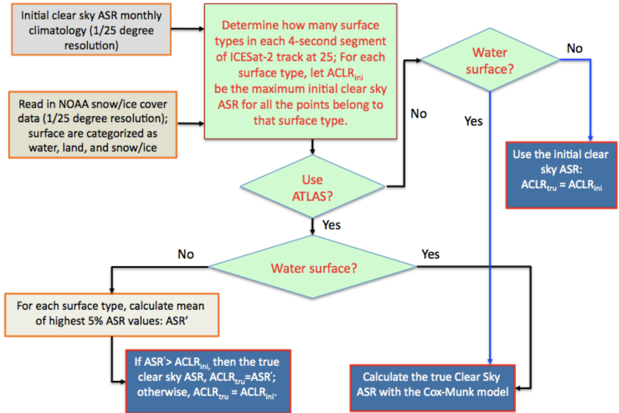
Figure 4.6.7. Flow chart for the clear sky ASR determination for every four seconds of data.
