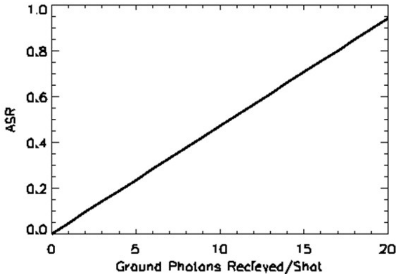
Figure 4.6.1 The apparent surface reflectance as computed from Equation 4.7 as a function of the number of surface return photons received per laser pulse. In practice, the ATLAS atmospheric data will be the sum of 400 laser pulses, and thus the photons received 400 times larger.
