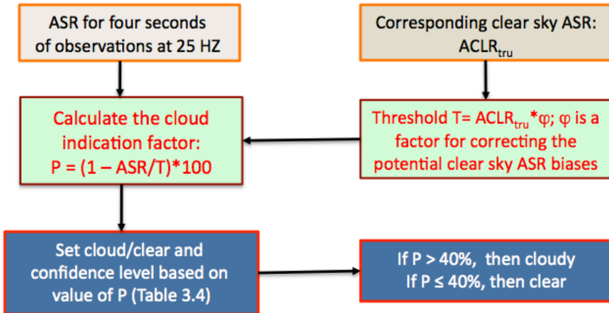
Figure 4.6.9. Flow chart for cloud determination for four seconds of data after the clear sky ASR is determined.
