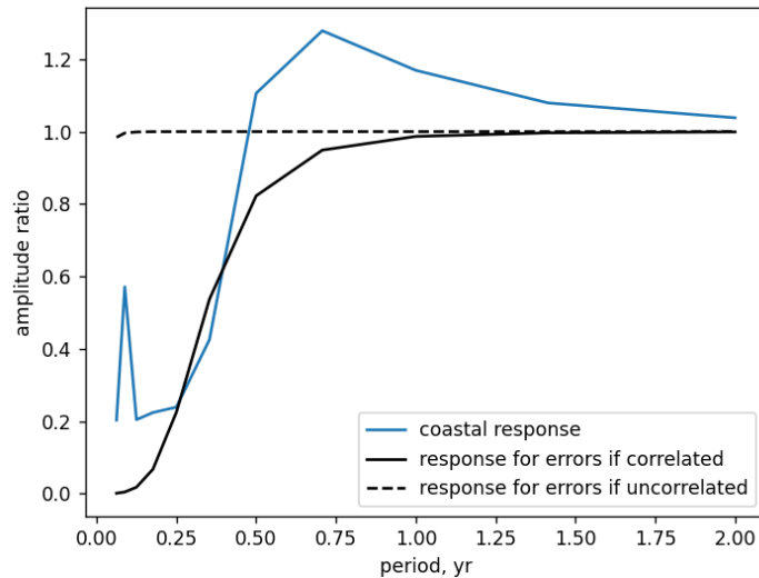
Figure 9. Analytic and computed amplitude response to sinusoidal signals.
