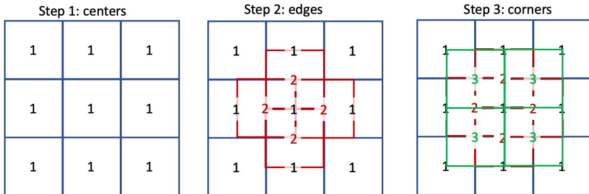
Figure 5. Tiling scheme. In step 1, data are loaded into non-overlapping 80x80 km tiles. In step 2, data are reloaded from the tiles in step 1, preserving the data editing. In step 3, data are loaded from the tiles in steps 1 and 2.
