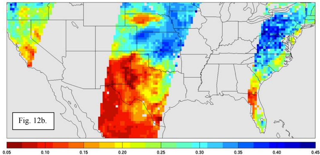
Figure 12. Simulation of L3_SM_P retrieved soil moisture in \text{cm}^3/\text{cm}^3 . This example is based on the single channel algorithm operating on H-polarized T_B observations simulated using geophysical data from a land surface model.
